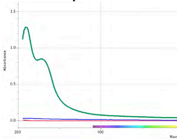
Far-UV Absorption
